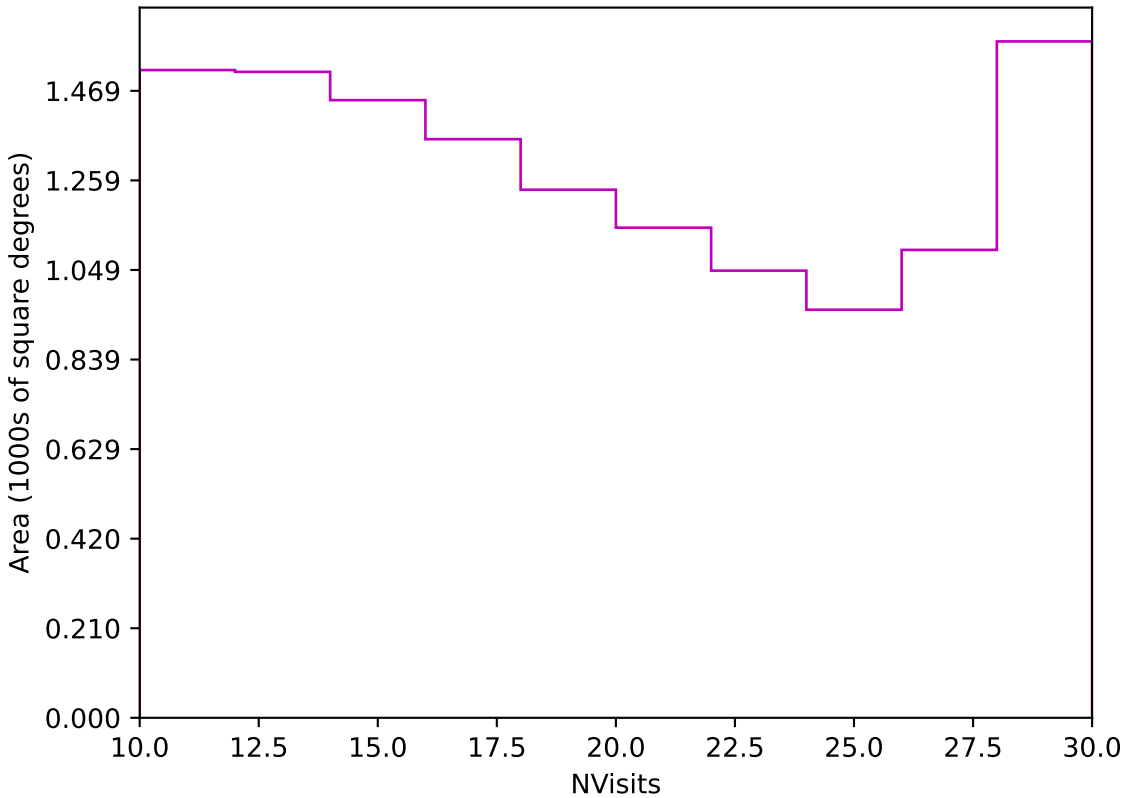
weather_cloudso16v3.4_10yrs Yr 3-4 z band: NVisits
