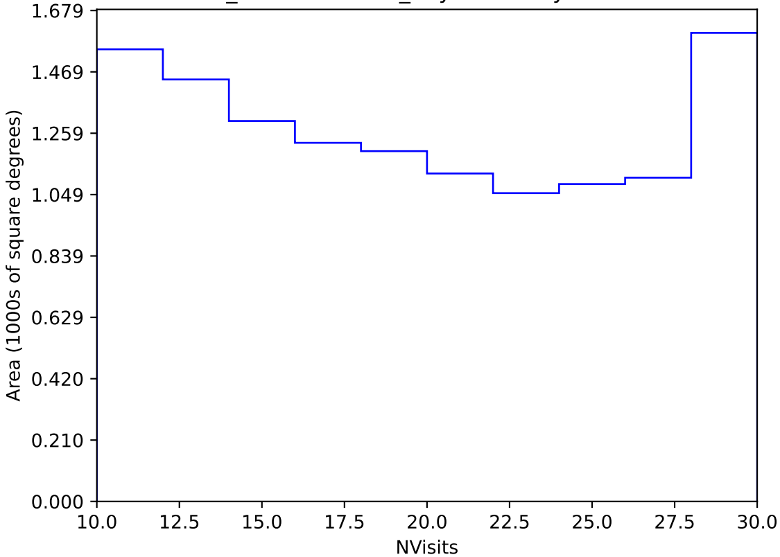
weather_cloudso16v3.4_10yrs Yr 3-4 y band: NVisits
