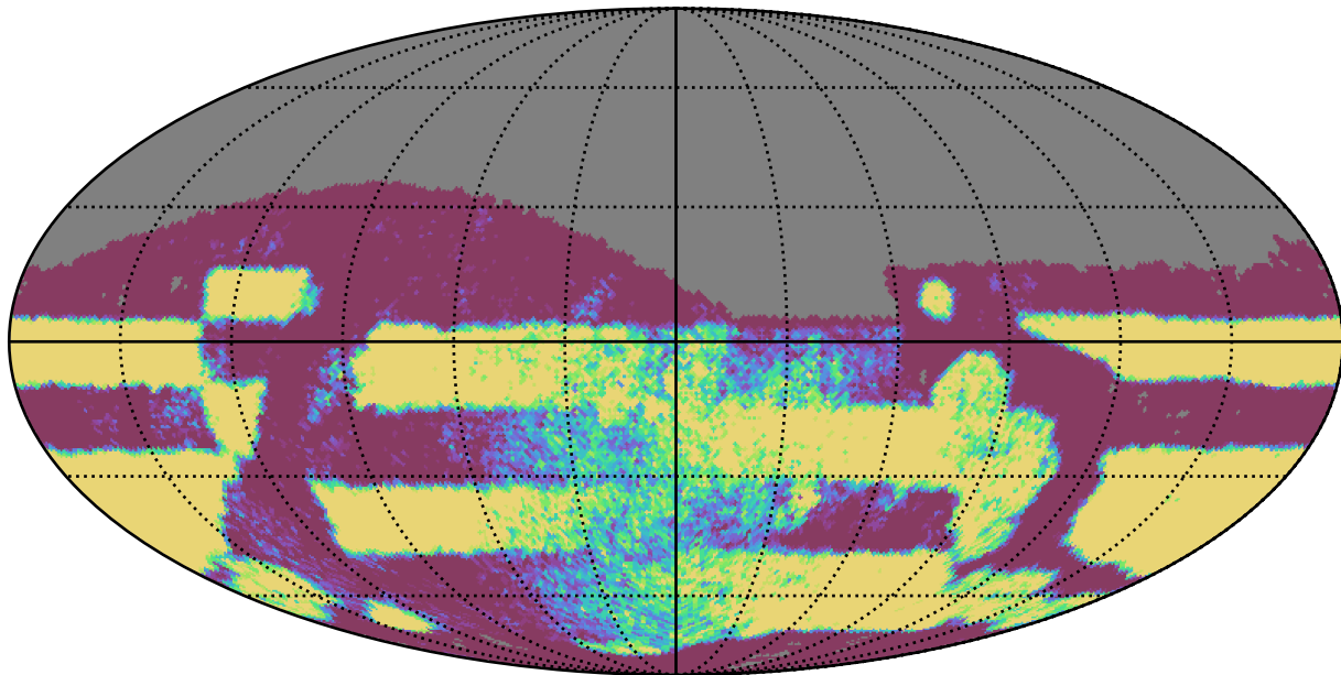
weather_cloudso16v3.4_10yrs Yr 3-4 r band: NVisits
