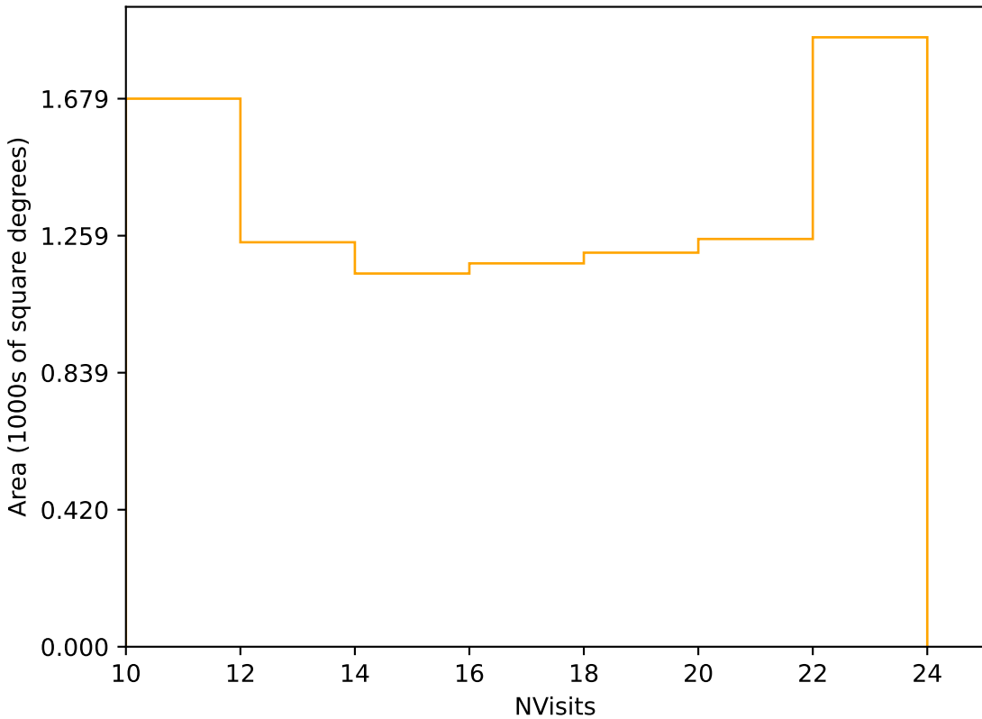
weather_cloudso16v3.4_10yrs Yr 3-4 r band: NVisits
