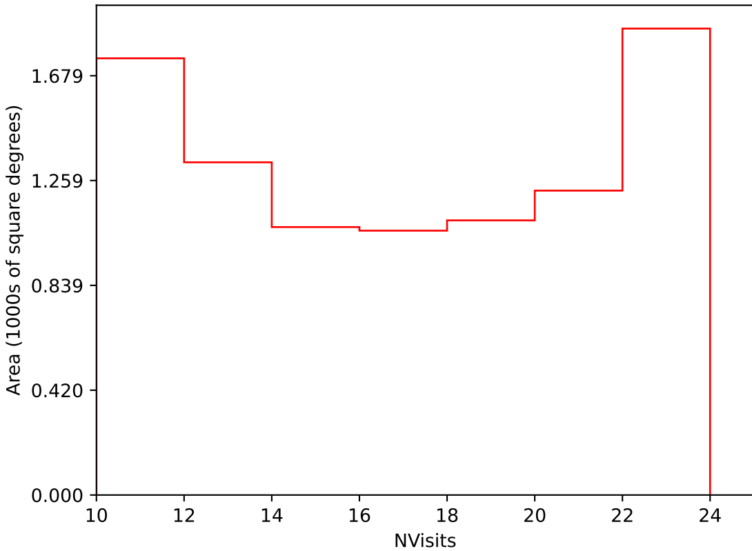
weather_cloudso16v3.4_10yrs Yr 3-4 i band: NVisits
