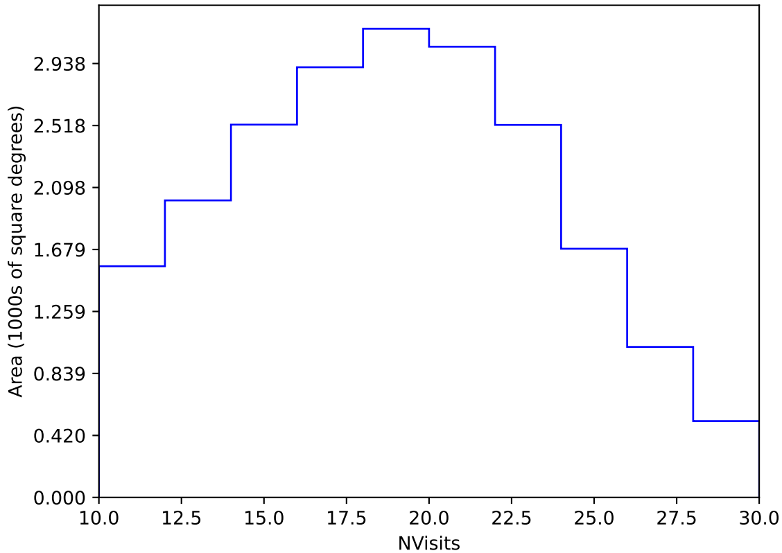
weather_cloudso16v3.4_10yrs Yr 1 y band: NVisits
