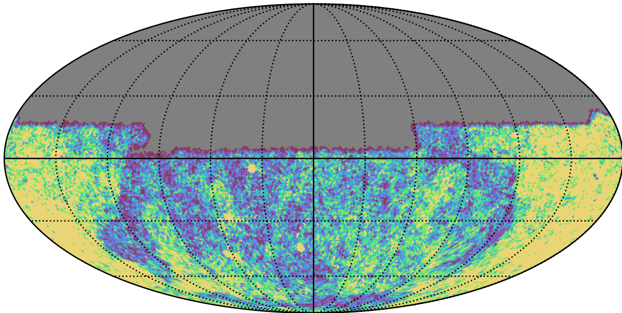
weather_cloudso16v3.4_10yrs Yr 1 u band: NVisits
