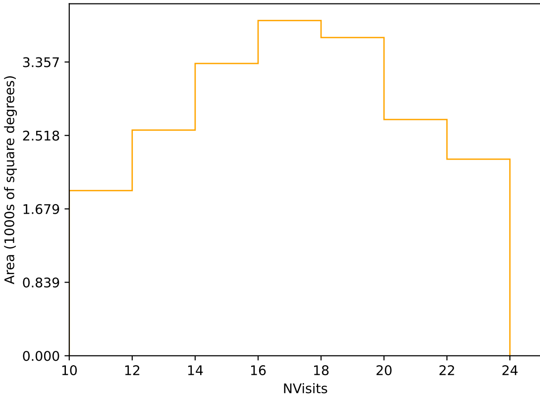
weather_cloudso16v3.4_10yrs Yr 1 r band: NVisits
