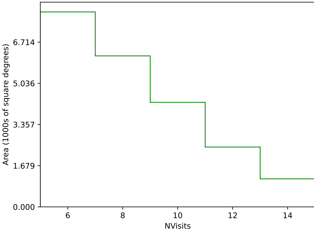
weather_cloudso16v3.4_10yrs Yr 1 g band: NVisits
