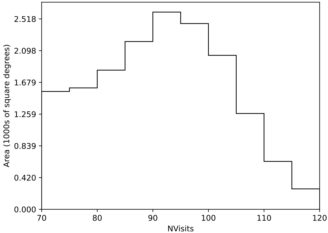
weather_cloudso16v3.4_10yrs Yr 1 all bands: NVisits
