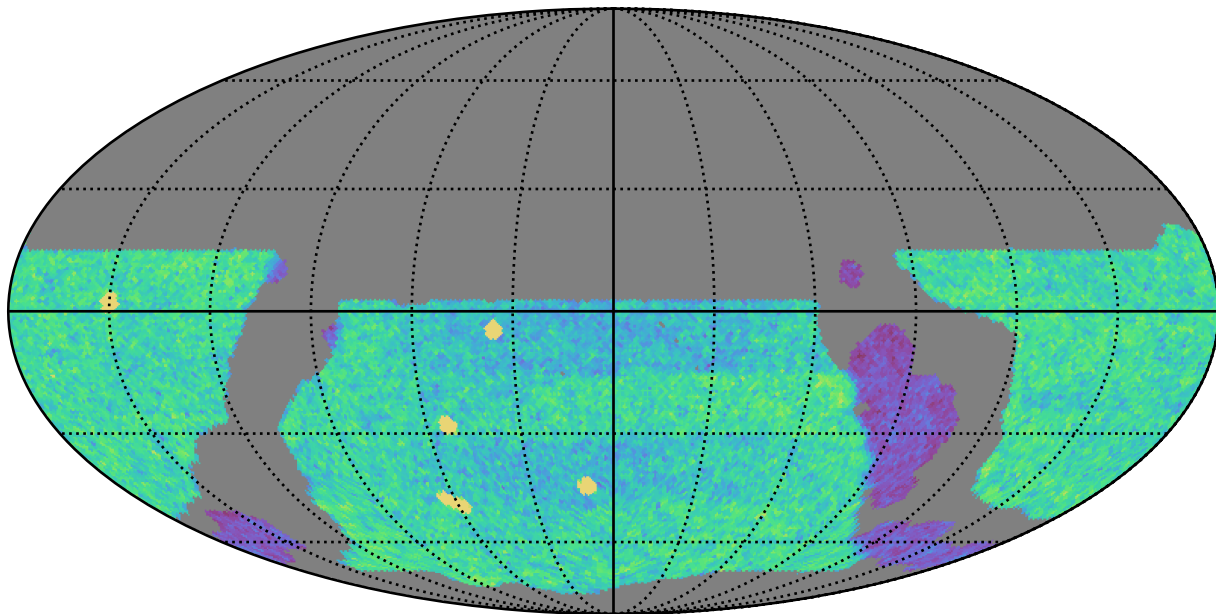
weather_cloudso16v3.4_10yrs WFD u band: NVisits
