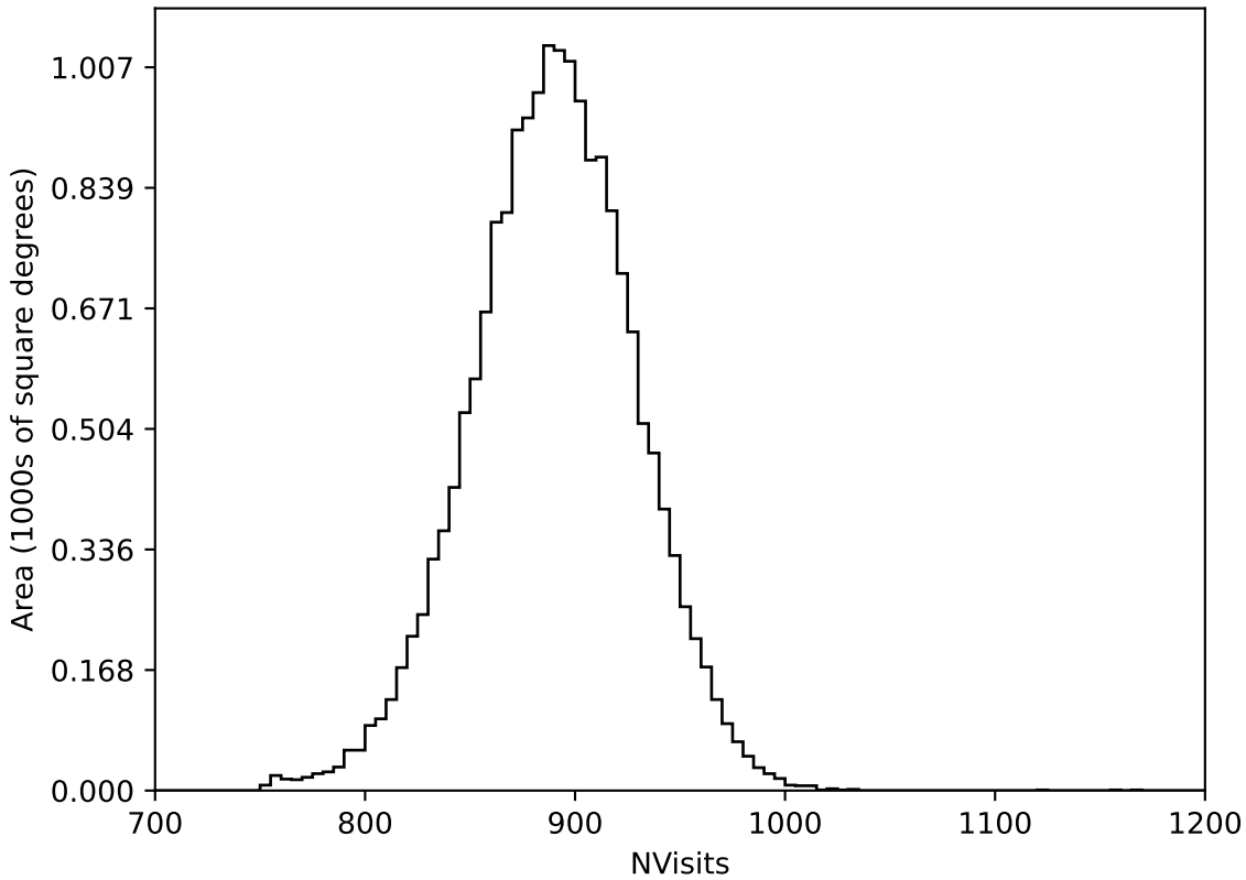
weather_cloudso16v3.4_10yrs WFD all bands: NVisits
