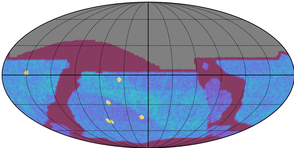
weather_cloudso16v3.4_10yrs All sky z band: NVisits
