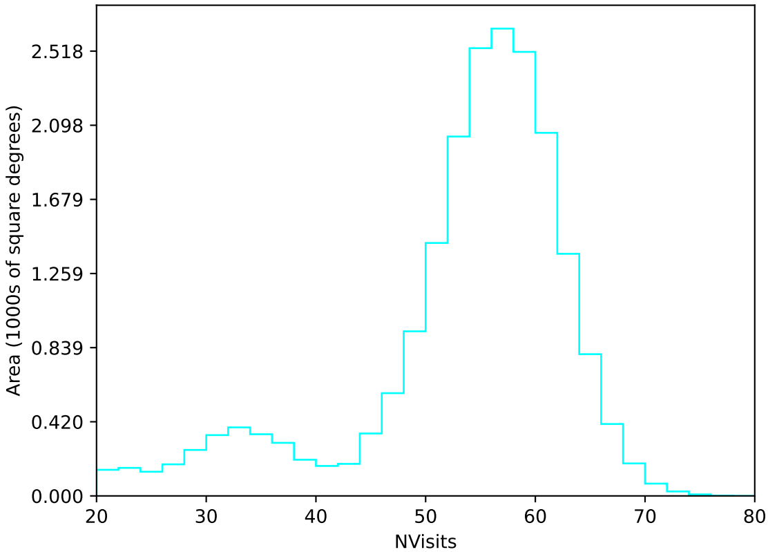
weather_cloudso16v3.4_10yrs All sky u band: NVisits
