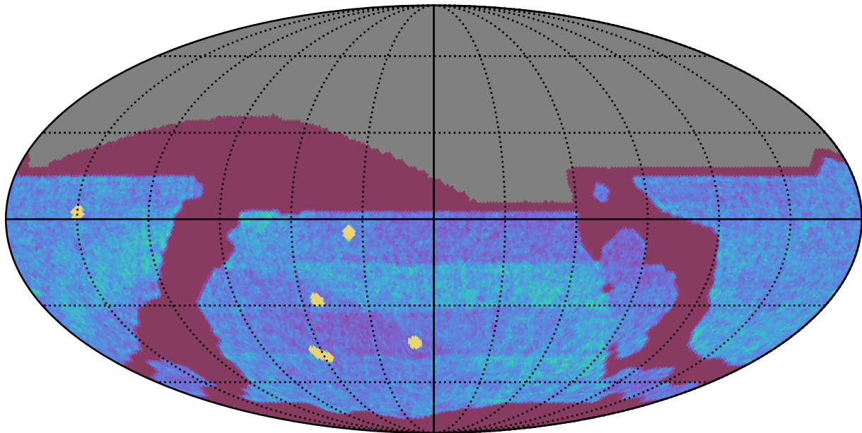
weather_cloudso16v3.4_10yrs All sky all bands: NVisits
