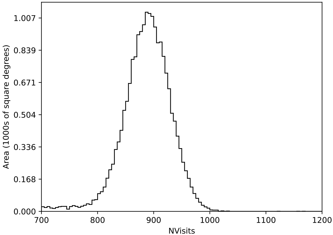
weather_cloudso16v3.4_10yrs All sky all bands: NVisits
