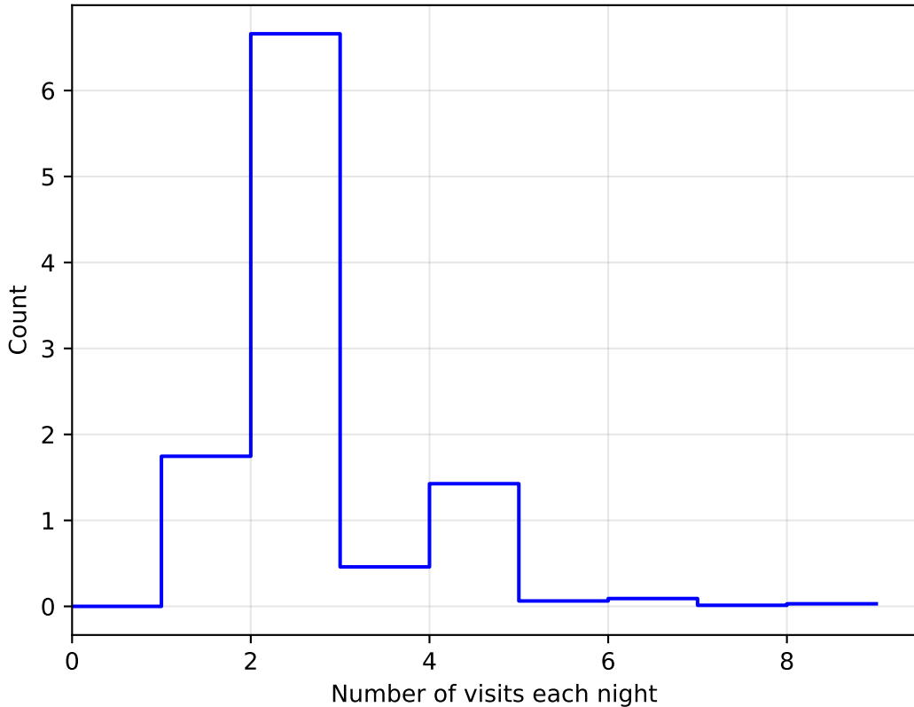
weather_cloudso16v3.4_10yrs All sky: NVisitsPerNight
