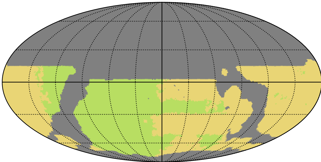
weather_cloudso16v3.4_10yrs WFD all bands: NSeasons
