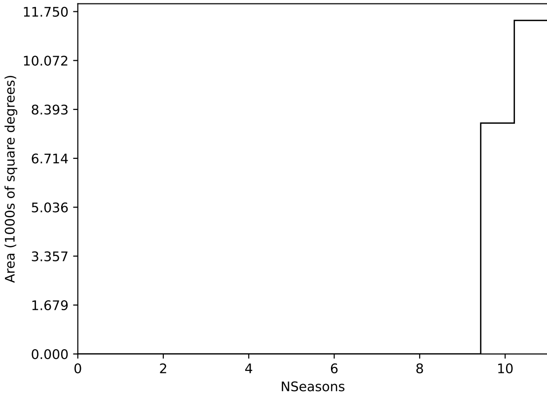
weather_cloudso16v3.4_10yrs WFD all bands: NSeasons
