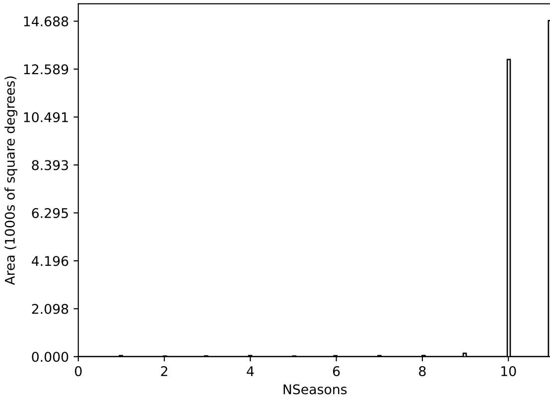
weather_cloudso16v3.4_10yrs All sky all bands: NSeasons
