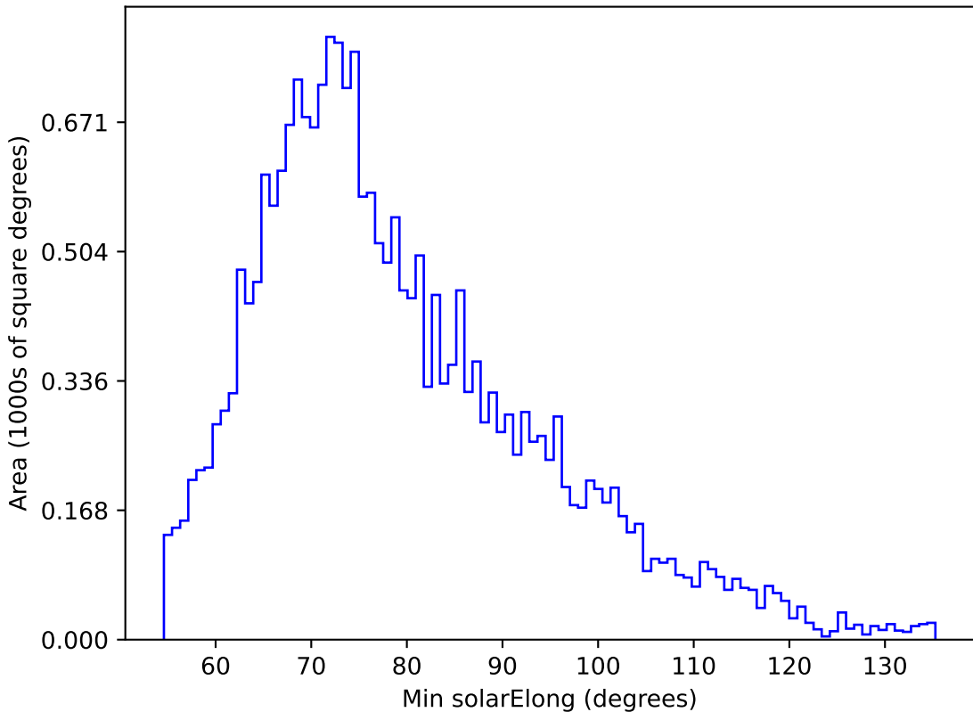
weather_cloudso16v3.4_10yrs All sky u band: Min solarElong
