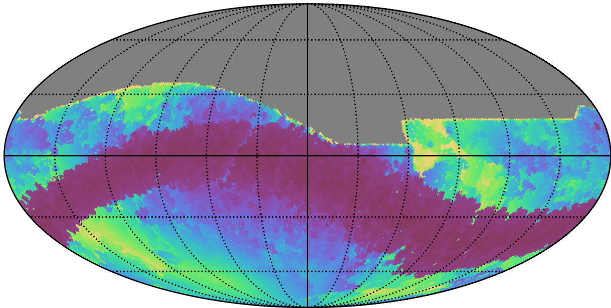
weather_cloudso16v3.4_10yrs All sky r band: Min solarElong
