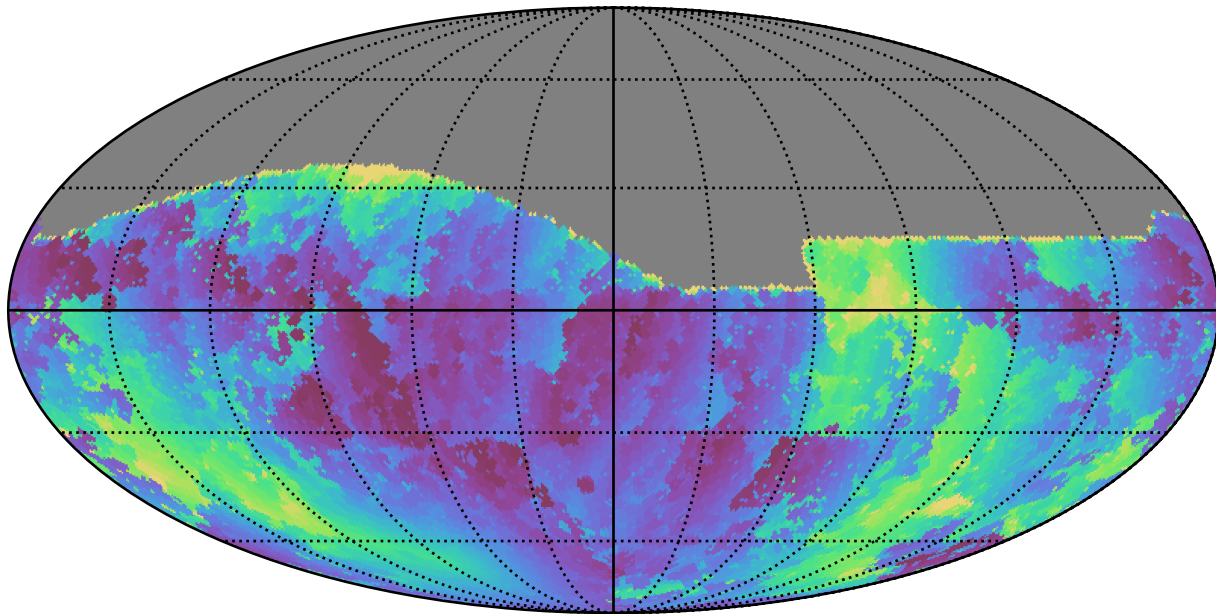
weather_cloudso16v3.4_10yrs All sky g band: Min solarElong
