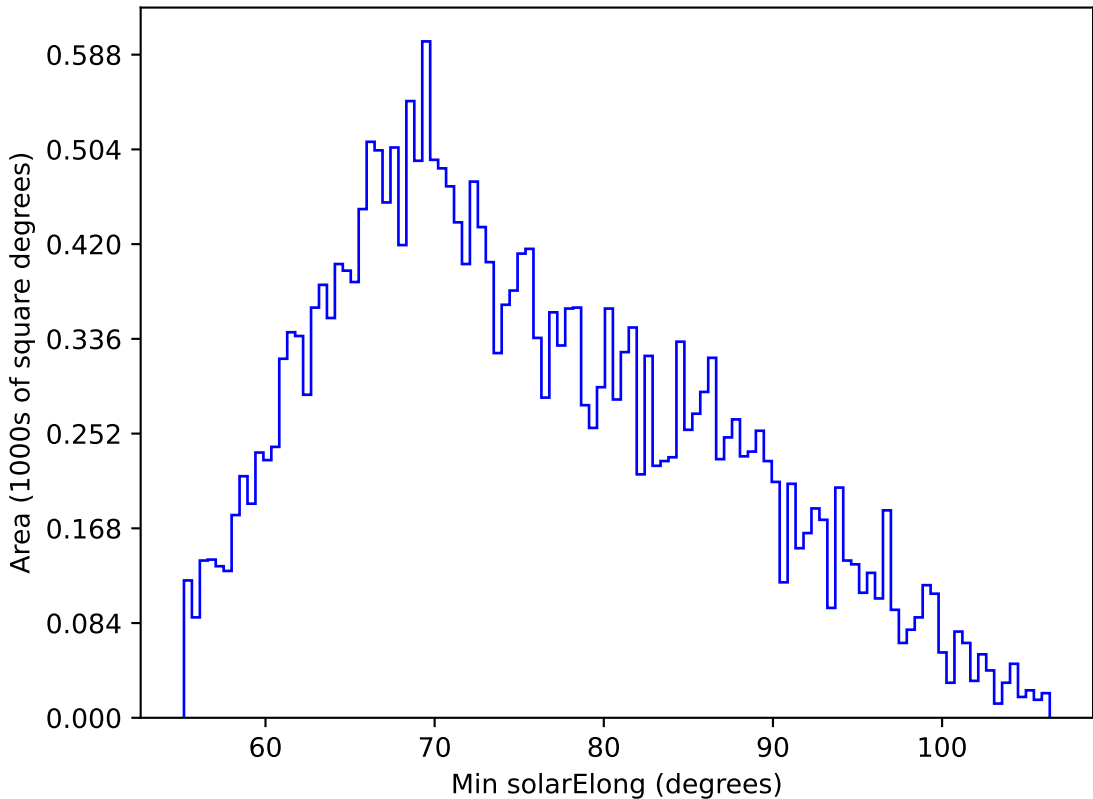
weather_cloudso16v3.4_10yrs All sky g band: Min solarElong
