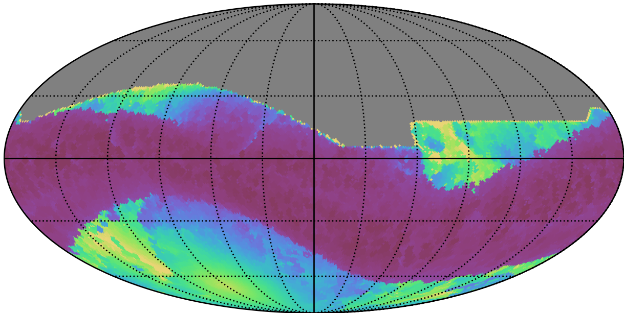
weather_cloudso16v3.4_10yrs All sky all bands: Min solarElong
