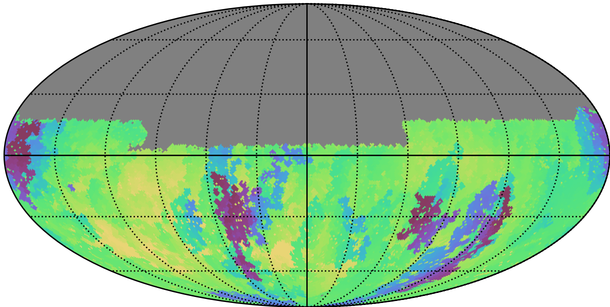
weather_cloudso16v3.4_10yrs Yr 1 u band: Min skyBrightness
