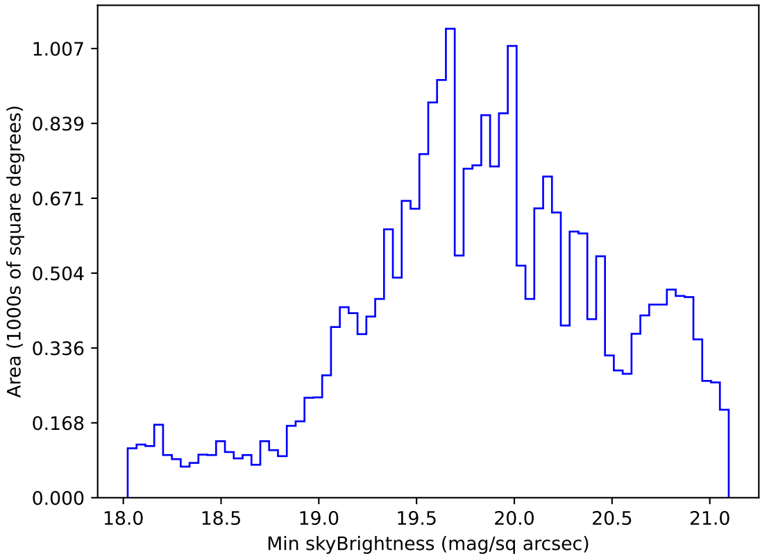
weather_cloudso16v3.4_10yrs Yr 1 r band: Min skyBrightness
