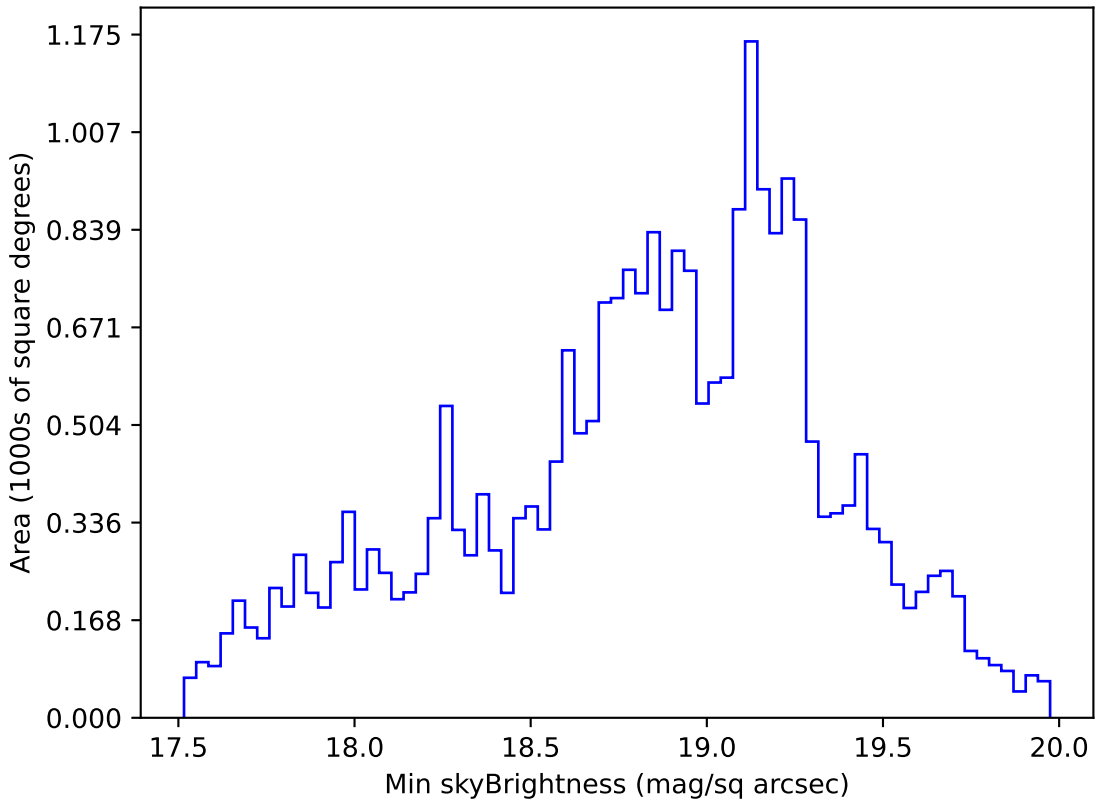
weather_cloudso16v3.4_10yrs Yr 1 i band: Min skyBrightness
