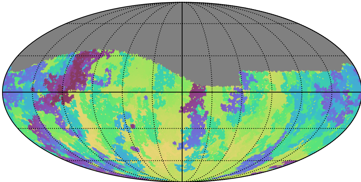
weather_cloudso16v3.4_10yrs Yr 1 g band: Min skyBrightness
