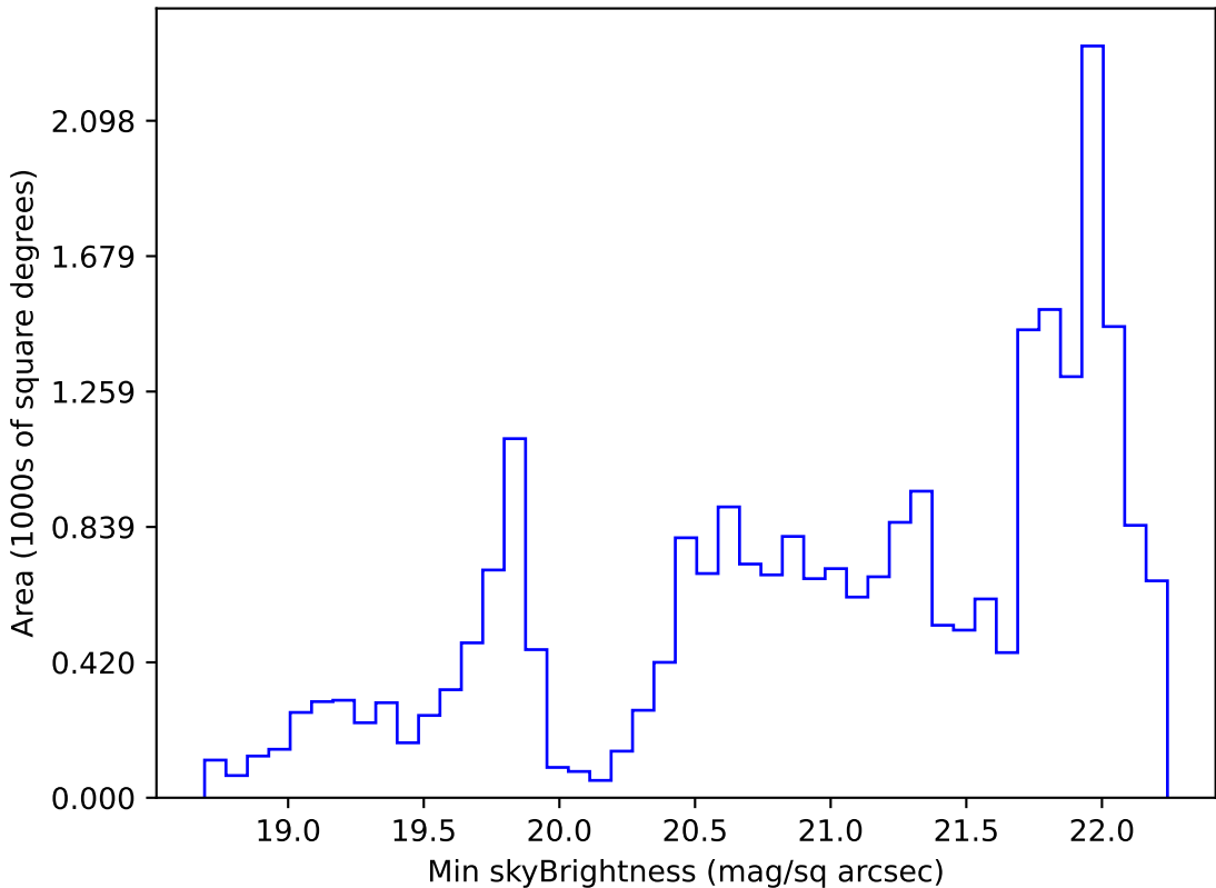
weather_cloudso16v3.4_10yrs Yr 1 g band: Min skyBrightness
