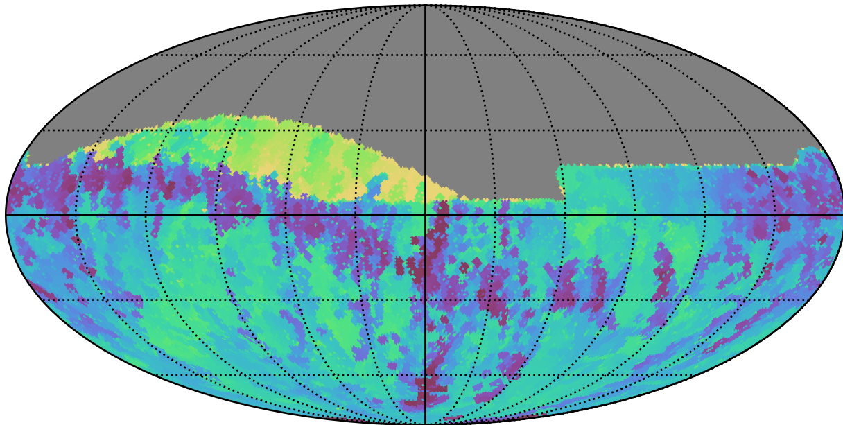
weather_cloudso16v3.4_10yrs Yr 1 all bands: Min skyBrightness
