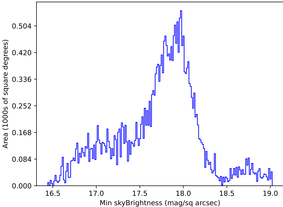
weather_cloudso16v3.4_10yrs Yr 1 all bands: Min skyBrightness
