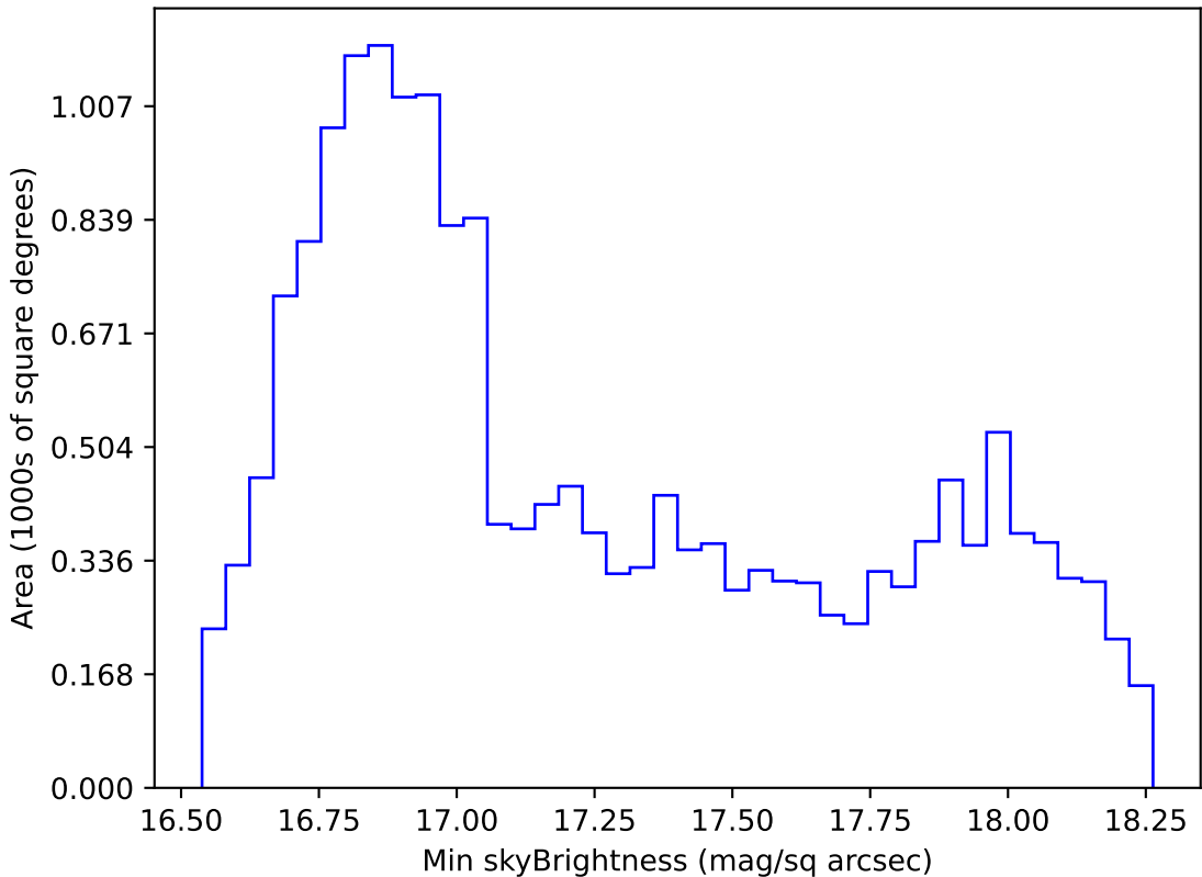
weather_cloudso16v3.4_10yrs WFD z band: Min skyBrightness
