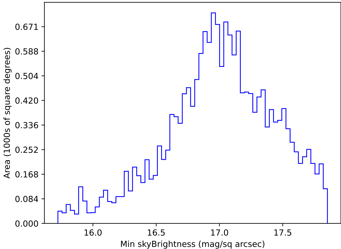
weather_cloudso16v3.4_10yrs WFD y band: Min skyBrightness
