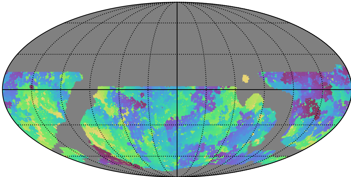
weather_cloudso16v3.4_10yrs WFD u band: Min skyBrightness
