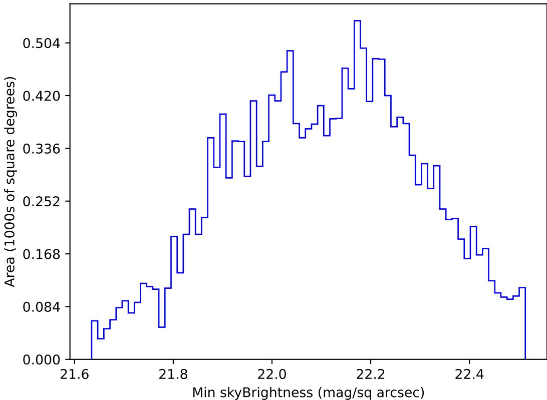
weather_cloudso16v3.4_10yrs WFD u band: Min skyBrightness
