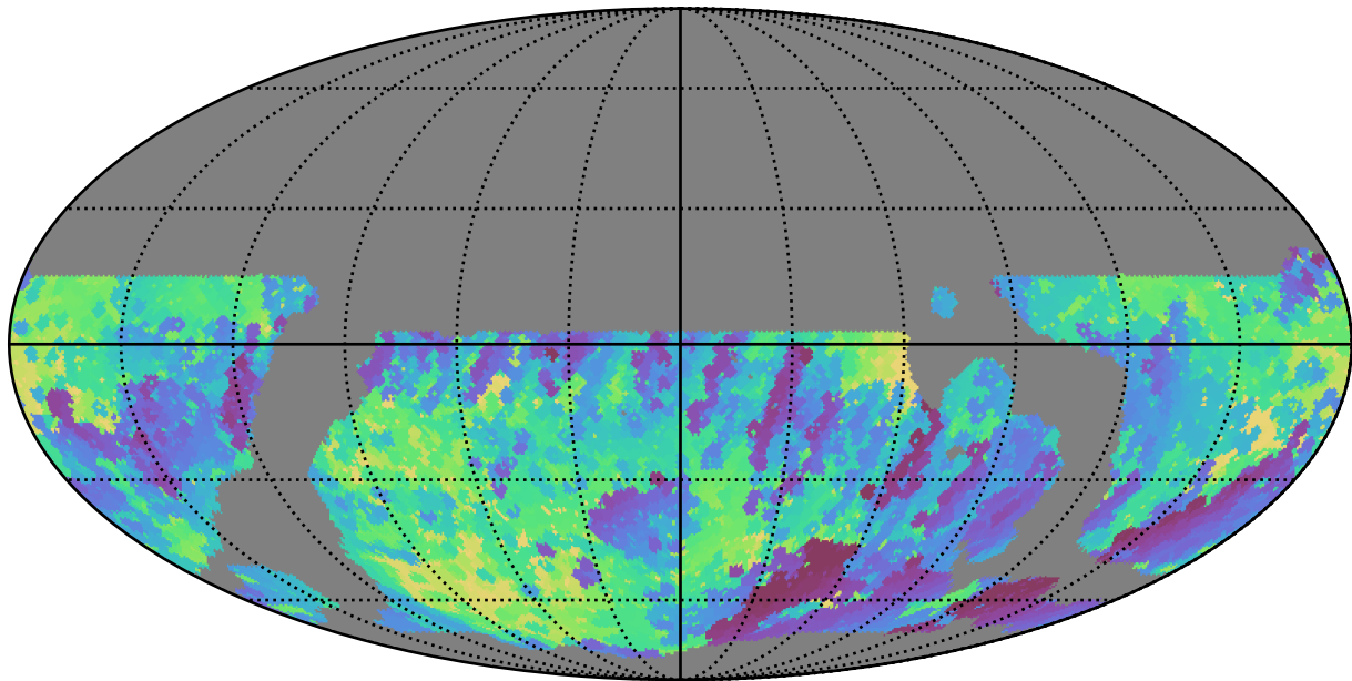
weather_cloudso16v3.4_10yrs WFD r band: Min skyBrightness
