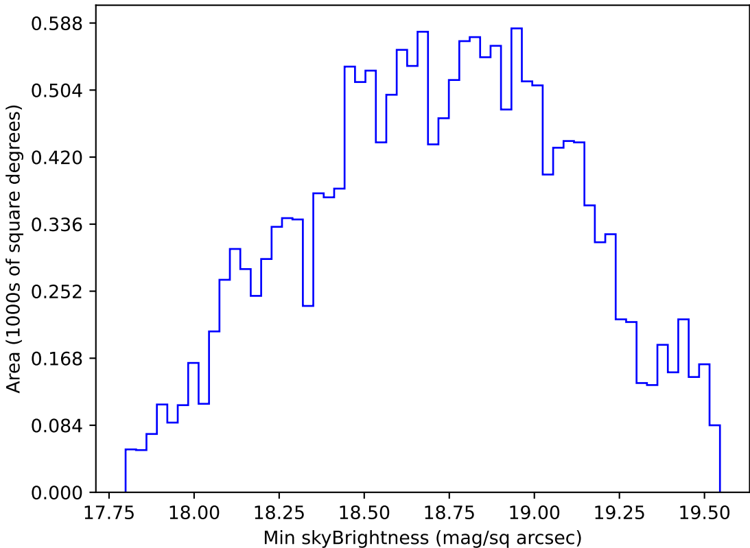
weather_cloudso16v3.4_10yrs WFD r band: Min skyBrightness
