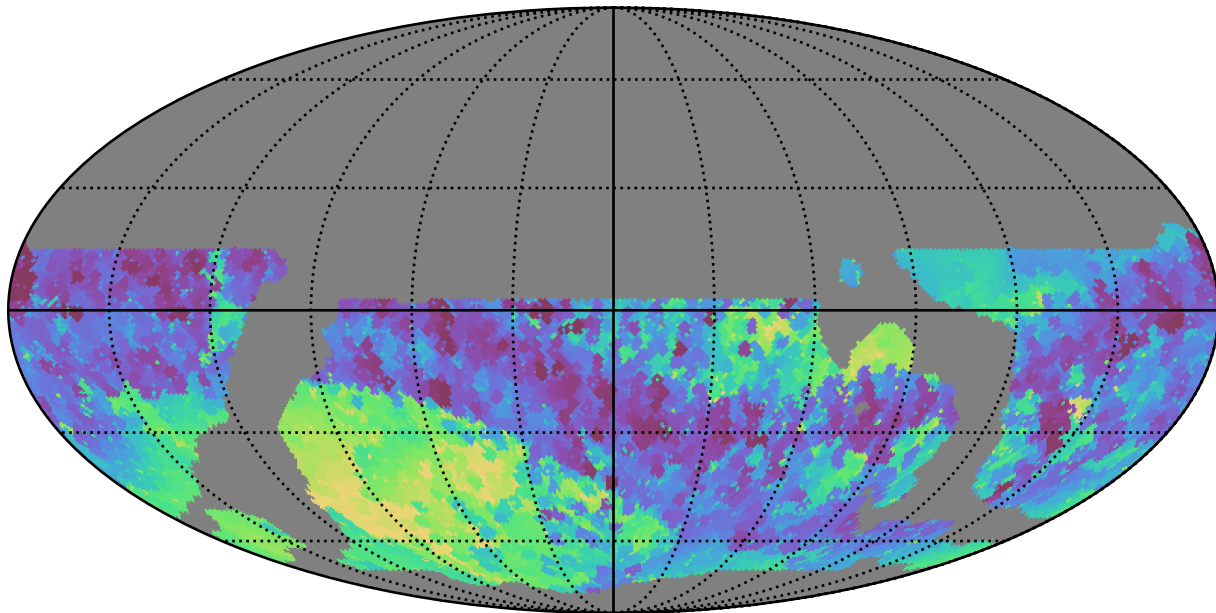
weather_cloudso16v3.4_10yrs WFD i band: Min skyBrightness
