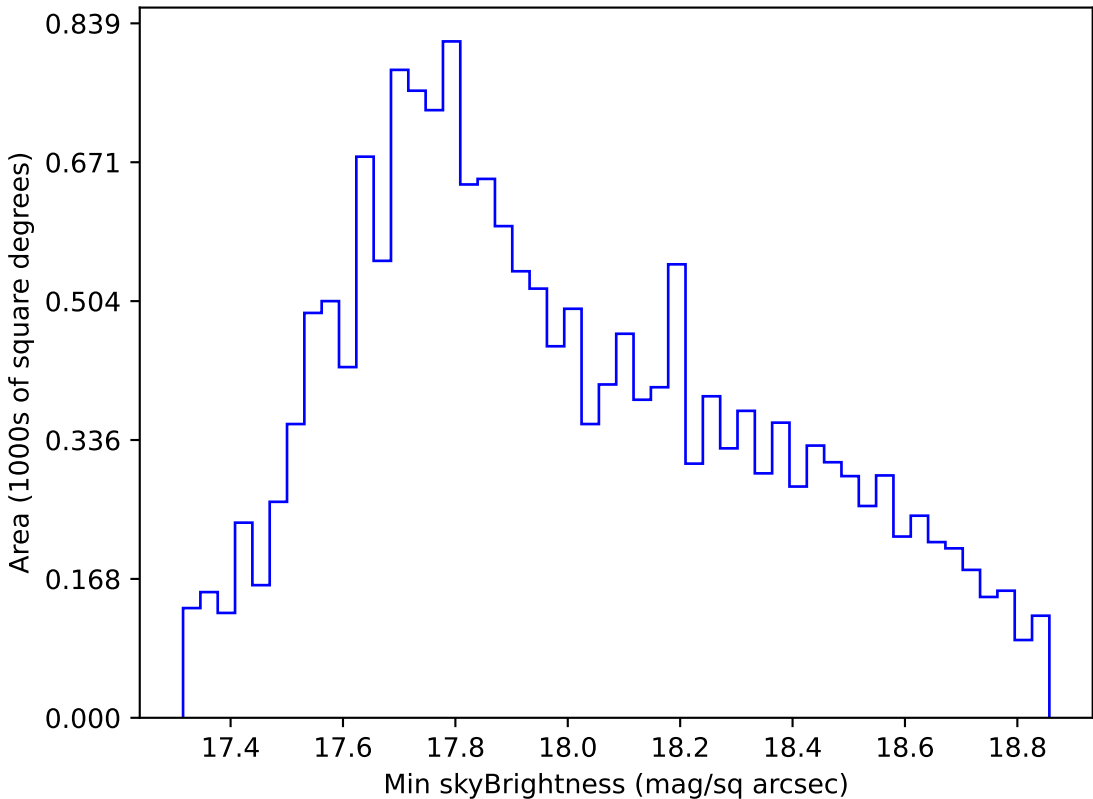
weather_cloudso16v3.4_10yrs WFD i band: Min skyBrightness
