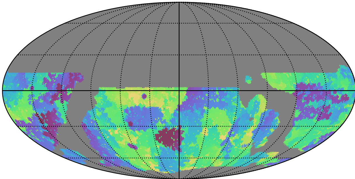
weather_cloudso16v3.4_10yrs WFD g band: Min skyBrightness
