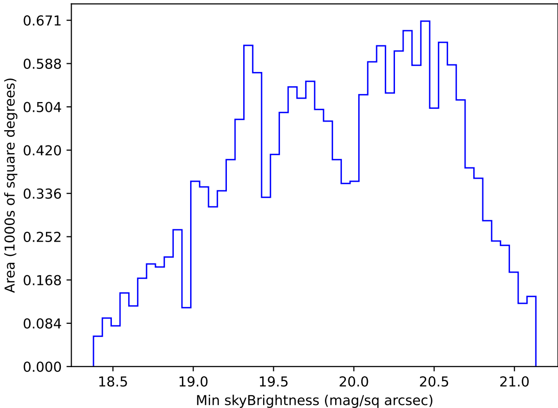
weather_cloudso16v3.4_10yrs WFD g band: Min skyBrightness
