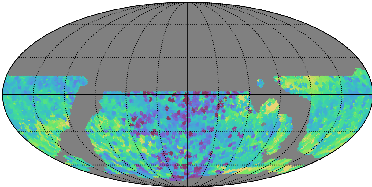
weather_cloudso16v3.4_10yrs WFD all bands: Min skyBrightness
