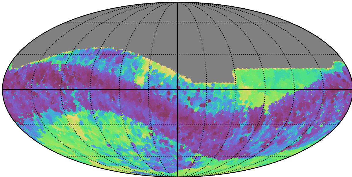
weather_cloudso16v3.4_10yrs All sky z band: Min skyBrightness
