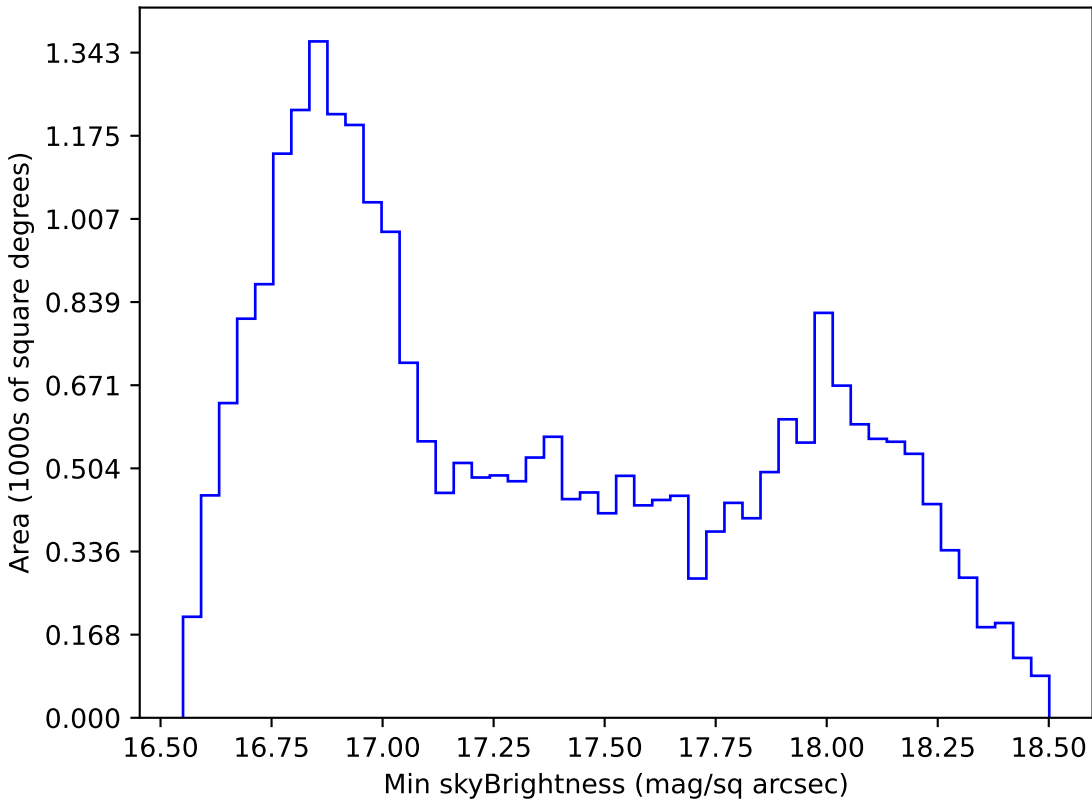
weather_cloudso16v3.4_10yrs All sky z band: Min skyBrightness
