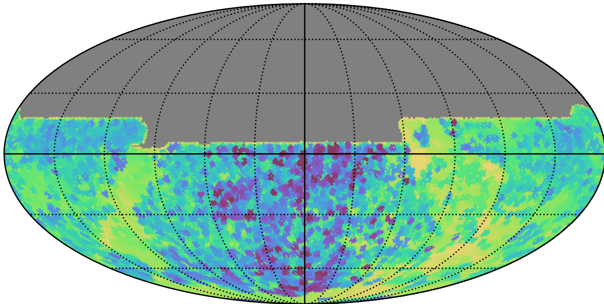
weather_cloudso16v3.4_10yrs All sky y band: Min skyBrightness
