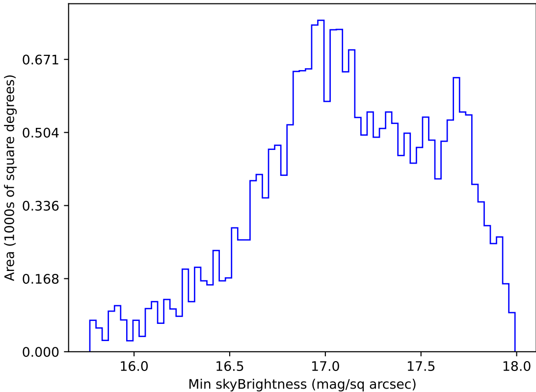
weather_cloudso16v3.4_10yrs All sky y band: Min skyBrightness
