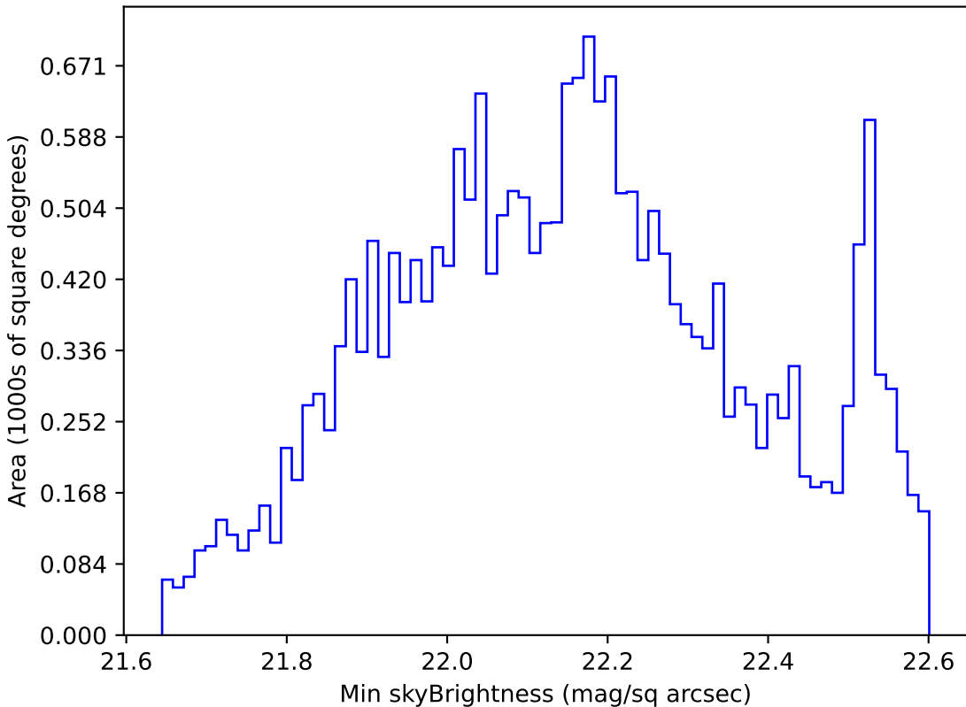
weather_cloudso16v3.4_10yrs All sky u band: Min skyBrightness
