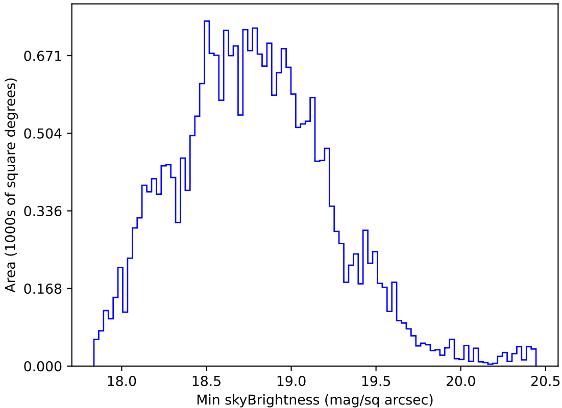
weather_cloudso16v3.4_10yrs All sky r band: Min skyBrightness
