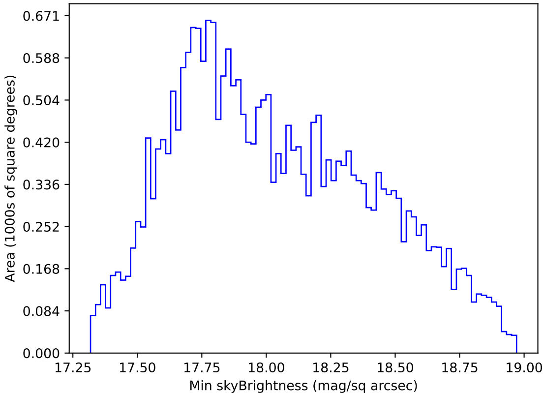
weather_cloudso16v3.4_10yrs All sky i band: Min skyBrightness
